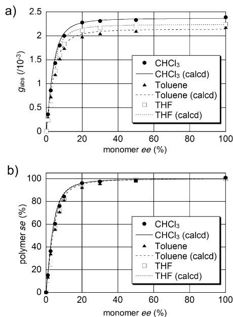
Figure 2. Correlation between the monomer ee value and the a) g_{\text{abs}} ( \Delta\epsilon/\epsilon at 362.5 nm) or b) se value of 2(x/y) (DP: 1000) in \text{CHCl}_3 , THF, or toluene.
